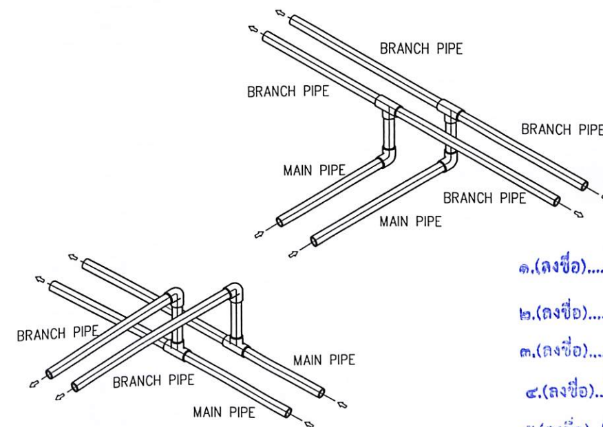
BRANCH PIPE INSTALLATION NOT TO SCALE
