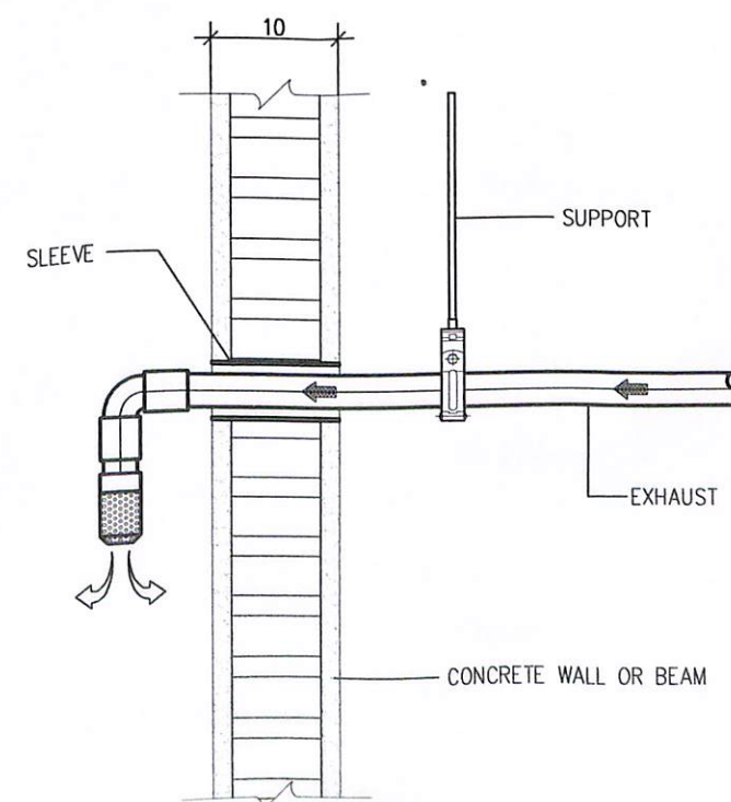
DETAIL OF SCAVENGE OUTLET (EXHAUST) NOT TO SCALE
