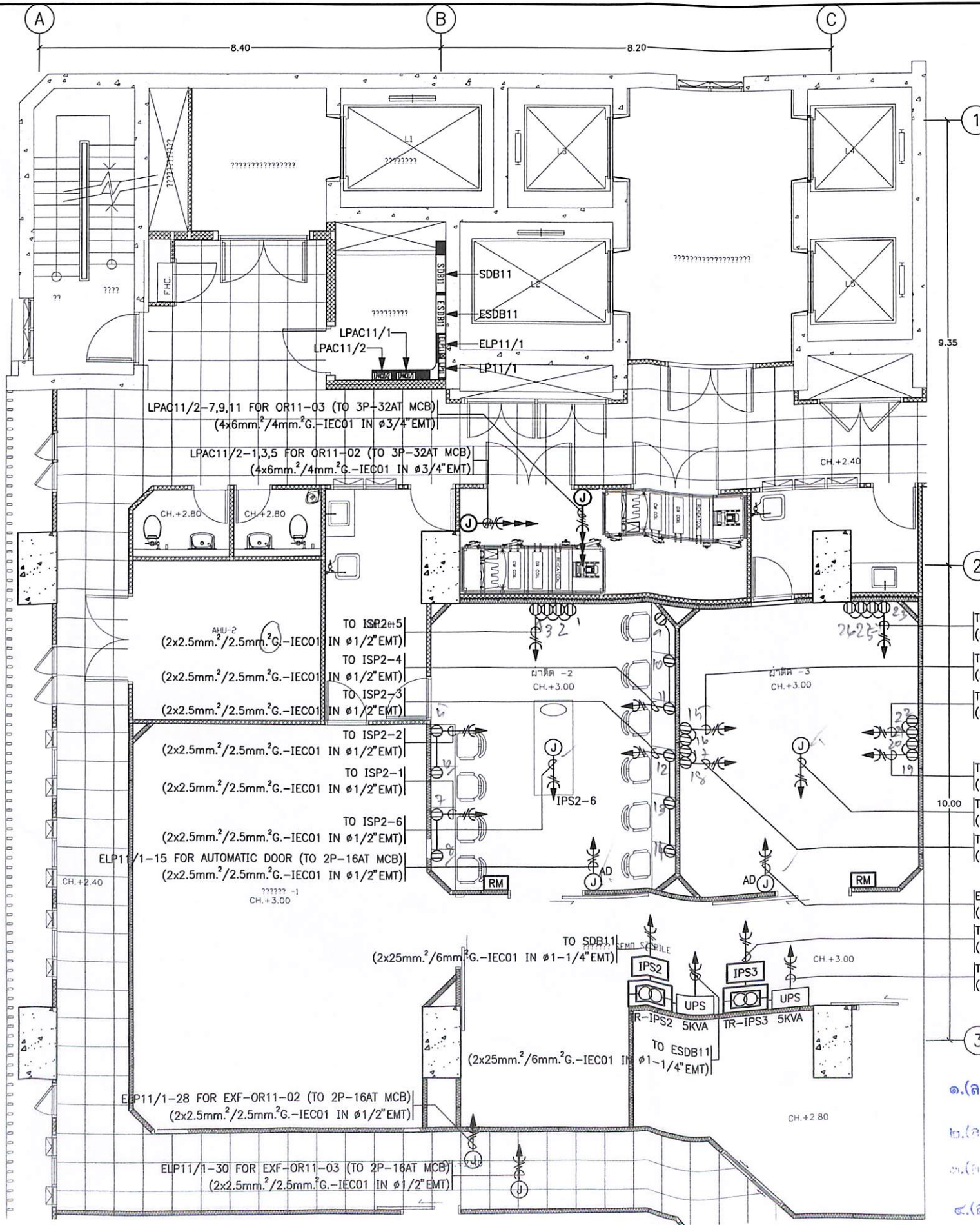
RECEPTACLE AND POWER OUTLET SYSTEM OPERATING (OR) ROOM 11th. FLOOR PLAN
