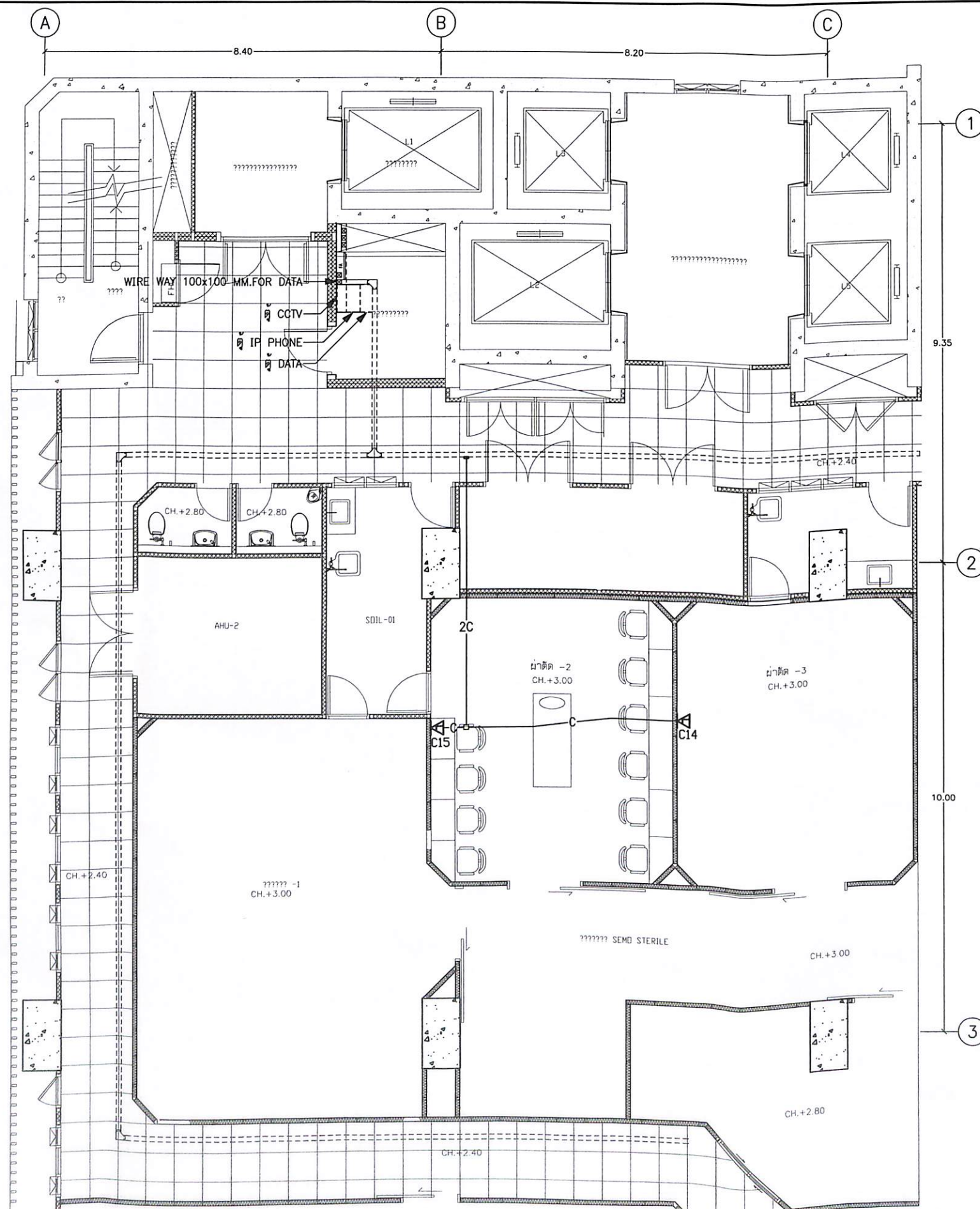
TELEPHONE, COMPUTER AND MATV SYSTEM OPERATING (OR) ROOM 11th. FLOOR PLAN SCALE 1:100
