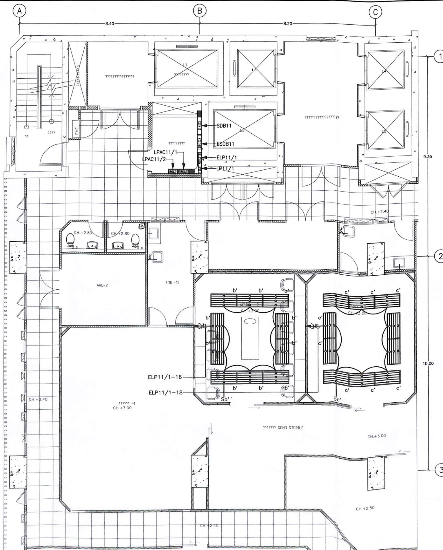
LIGHTING SYSTEM OPERATING (OR) ROOM 11th. FLOOR PLAN SCALE 1:100
